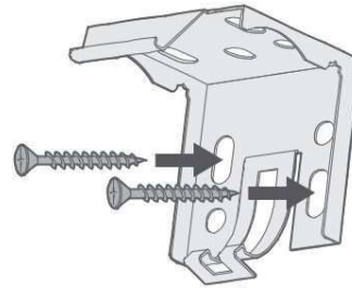
Face-Fixing
