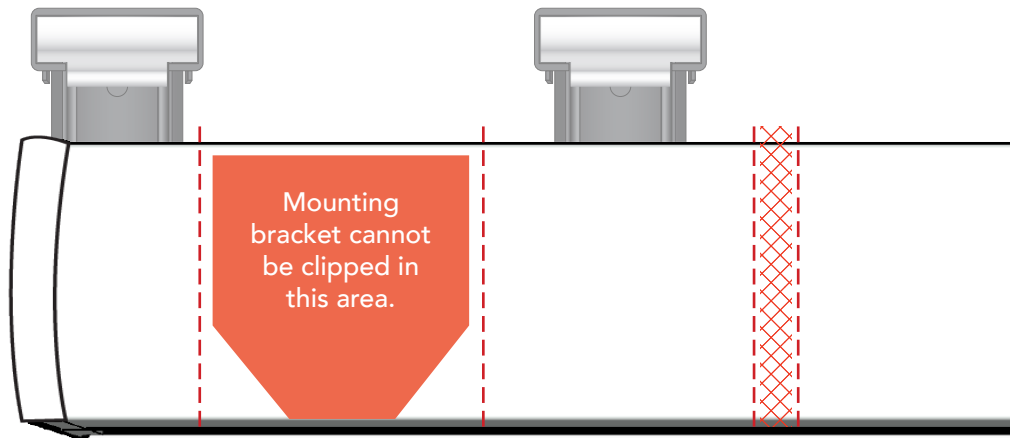
Front View of Headrail
