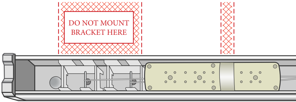
Top View of Headrail
