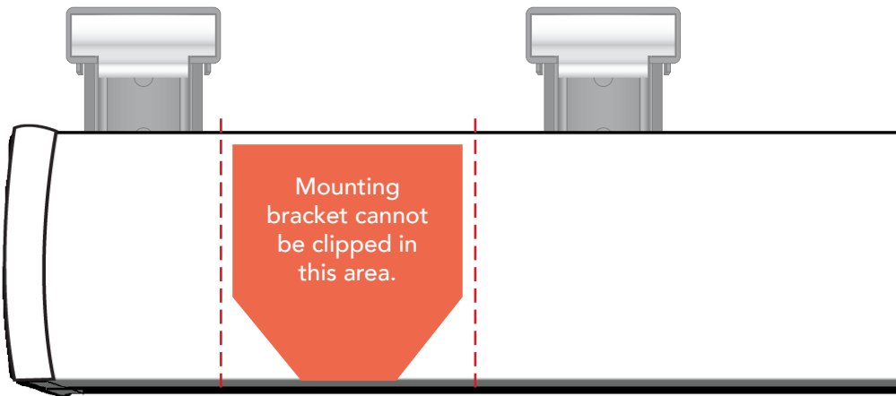
Front View of Headrail
